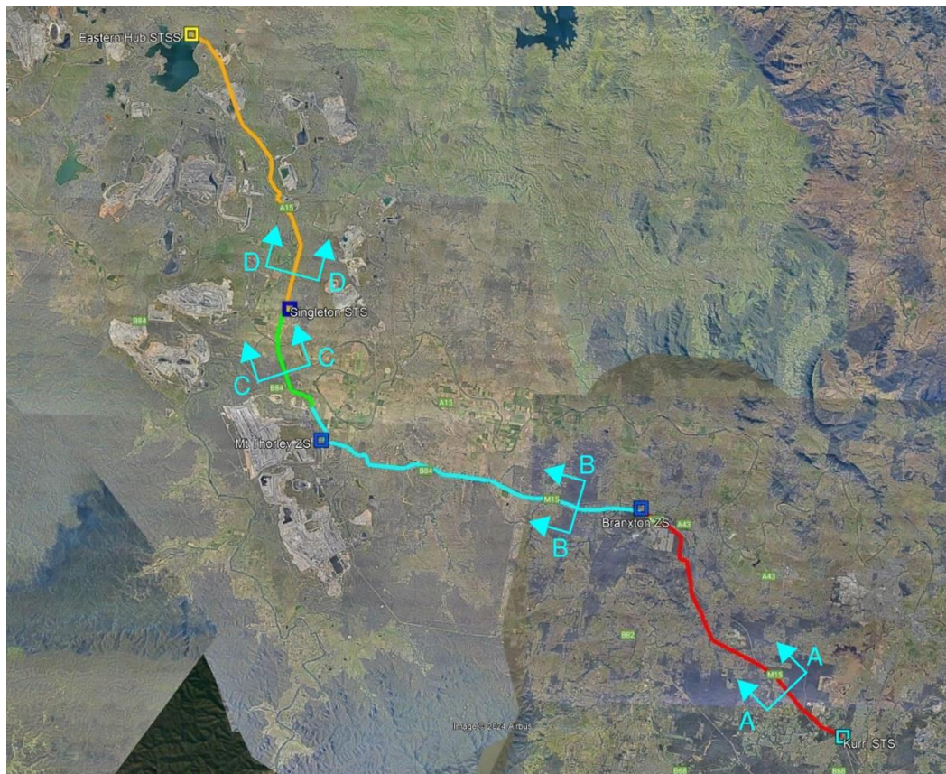
Figure 1-1 | Key components of the project from Kurri STS to Antiene Sub Transmission Substation (STSS) SS
