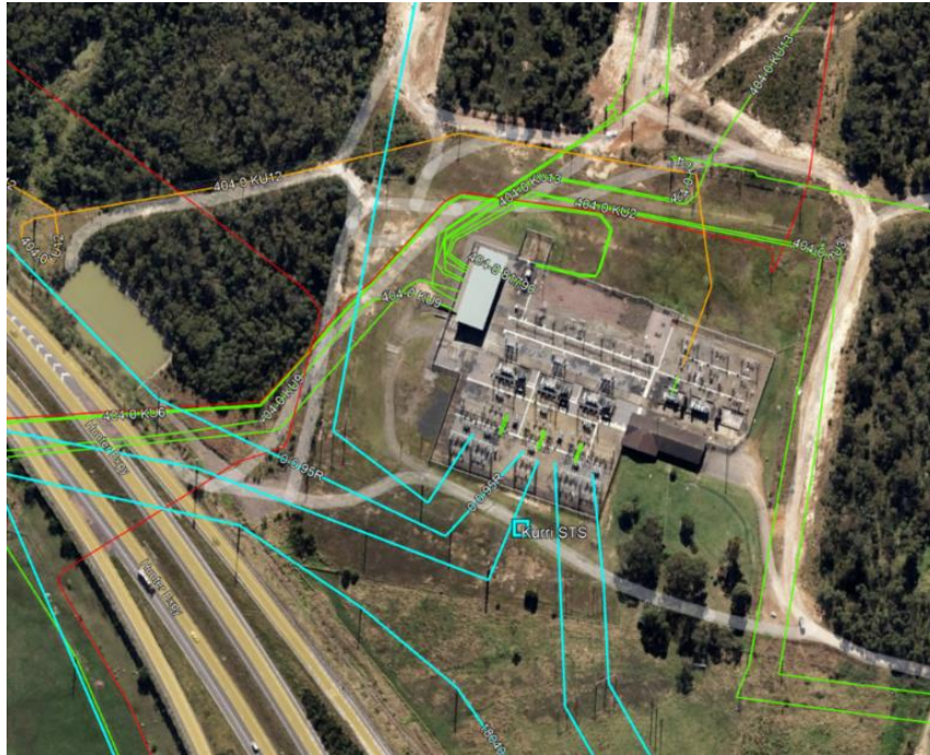
Figure 4-1 | Location of the existing Kurri STS
