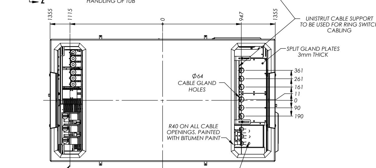
VIEW Y-Y VIEW FROM BELOW
