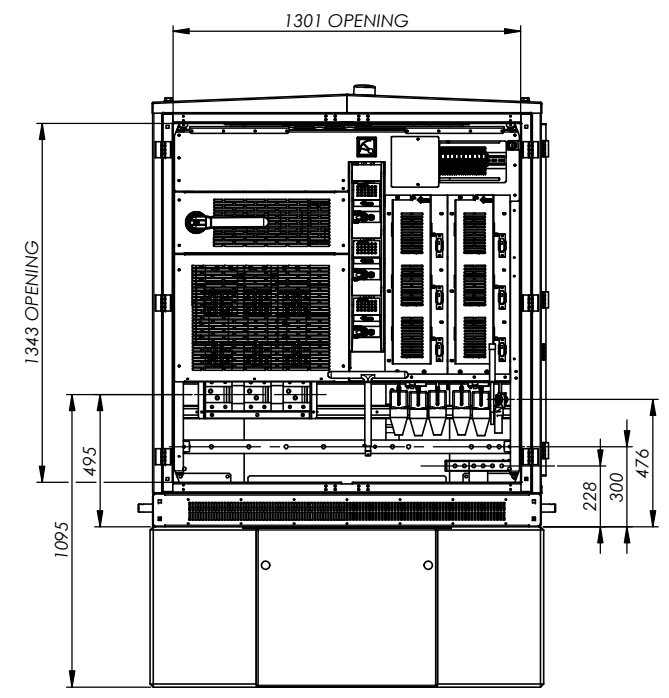
VIEW Z-Z 1200/1600A + 2x400A FEEDER ARRANGMENT SHOWN
