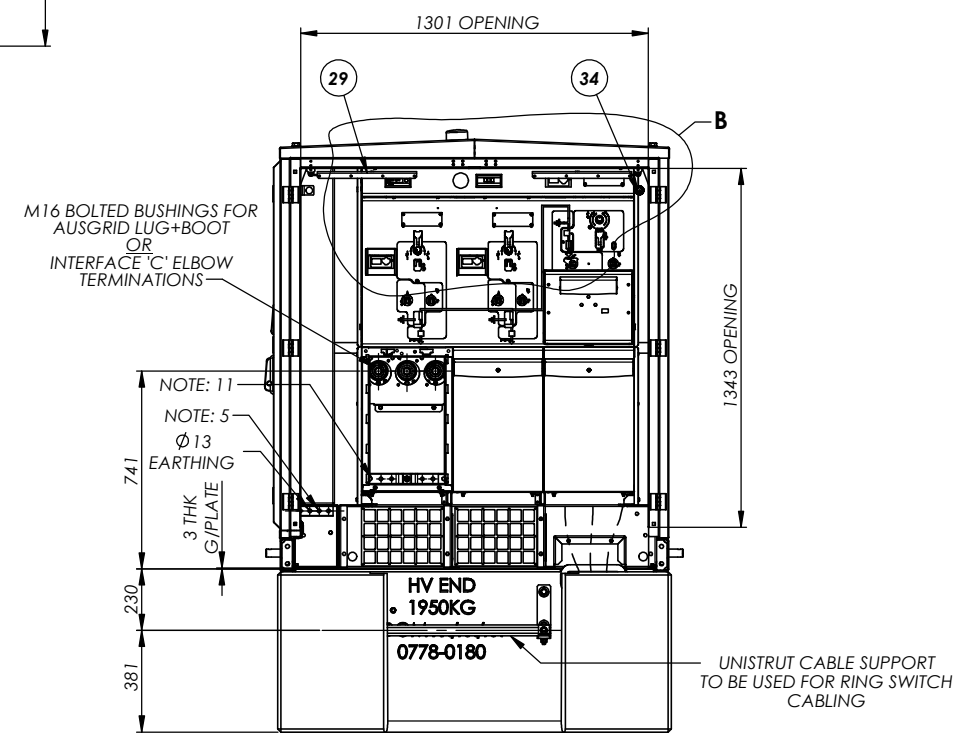
HV SIDE LHS END BOX COVER REMOVED ACCESS COVERS & END PANEL REMOVED
