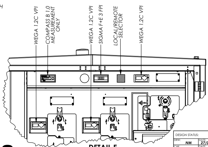
DETAIL E INSTRUMENT LAYOUT
