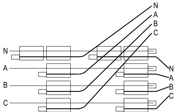
CONNECTION DIAGRAM
