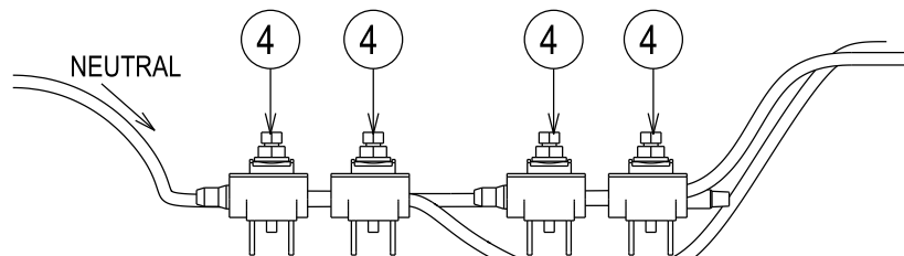
DETAIL 1
